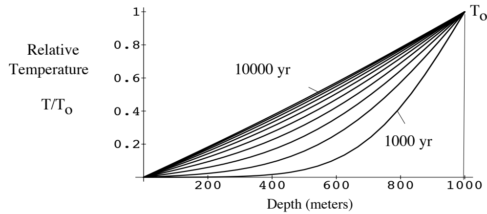
Figure 2. A slab is instantaneously heated at its bottom, and the analytic solution shows how the temperature evolves inside the slab for ten thousand years.
